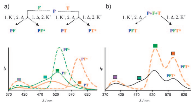
Figure 2. a) Four distinct emission patterns, corresponding to different receptor combinations, can be tuned by an appropriate choice of two ODNs and preparation methods. b) Different patterns generated by the three ODNs. Conditions: 570 nm P, 1.1 equiv F, and 1.1 equiv T, excited at 344 nm.
